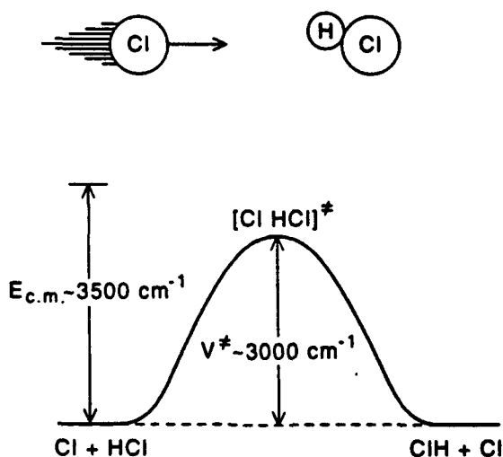
Fig. 10. Schematic of the Cl + HCl collision system for state-resolved energy transfer on open shell potential surfaces
